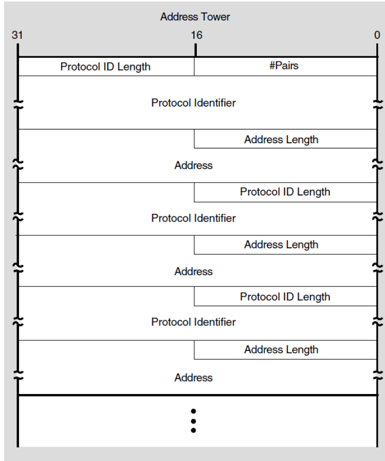
Figure 2.4. Protocol Tower Data Structure
