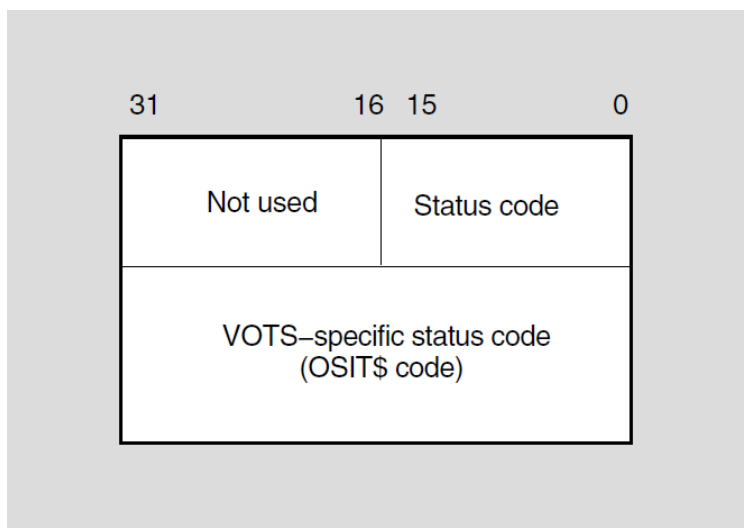
Figure C.5. IOSB with SS$_LINKABORT for Unsuccessful Read/Write $QIO(W)Calls
