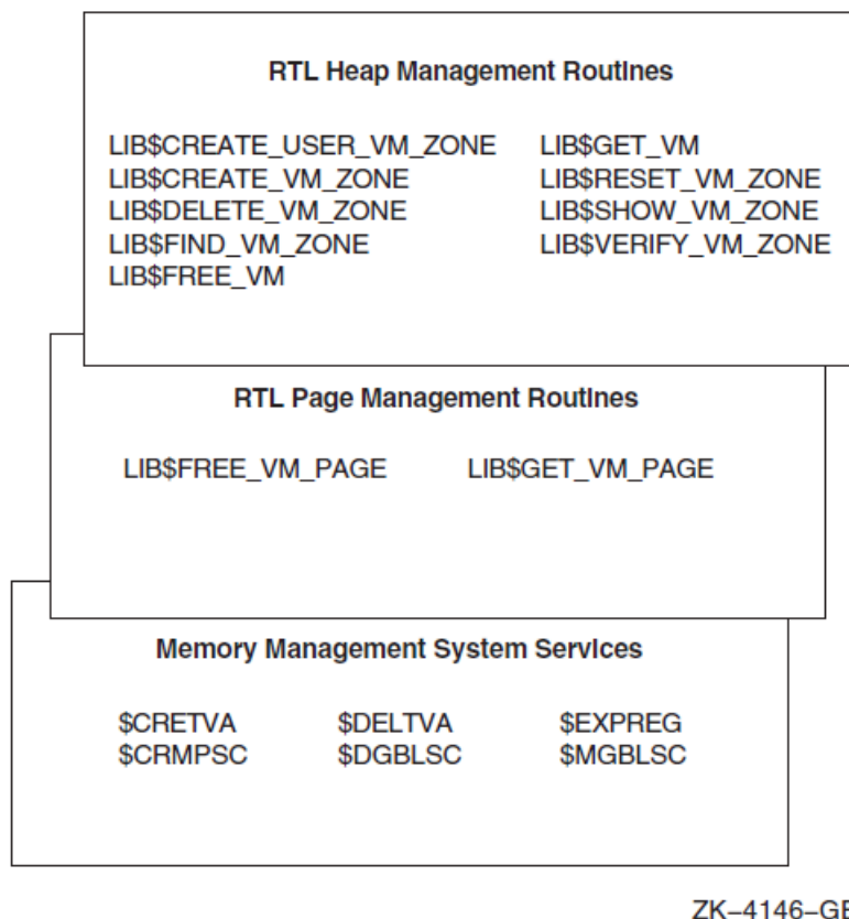
Figure 13.5. Hierarchy of VAX Memory Management Routines
