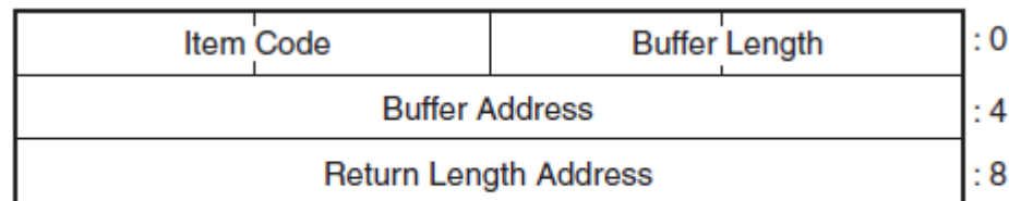
Figure 11.4. Item_list_3 Format
