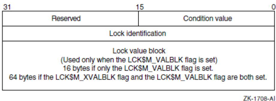
Figure 7.4. Lock Status Block
