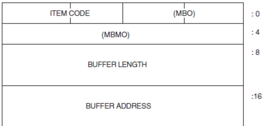
Figure 11.7. item_list_64a
