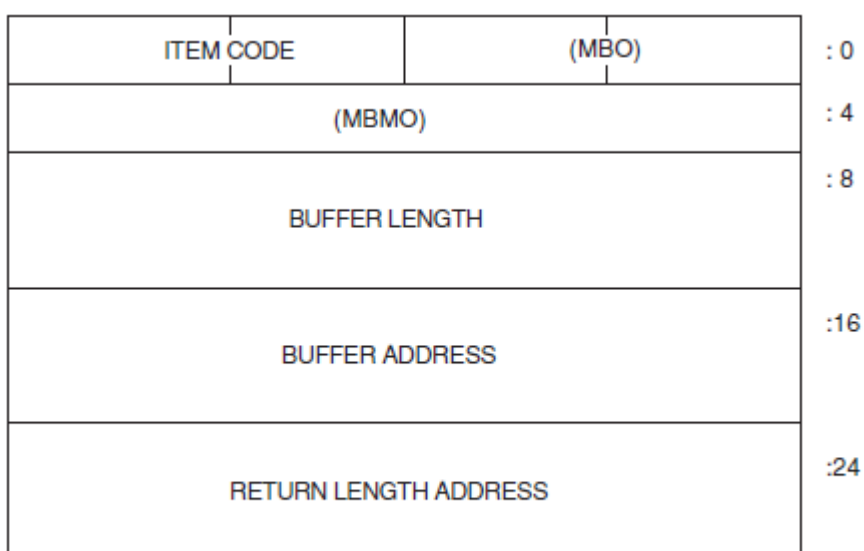
Figure 11.6. Item_list_64b Format
