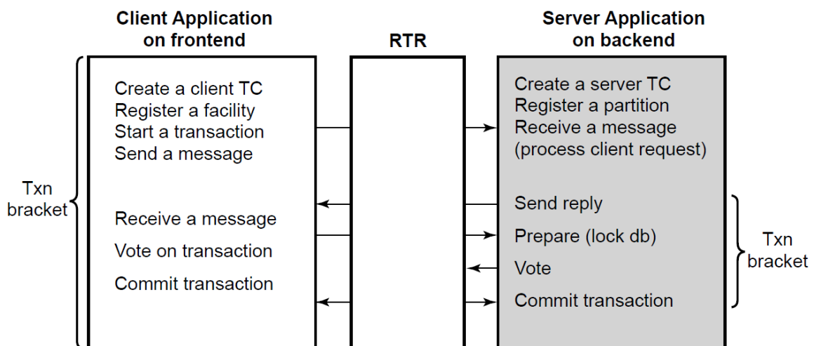
Figure 4.1. Transactional Messaging with the C++ API
