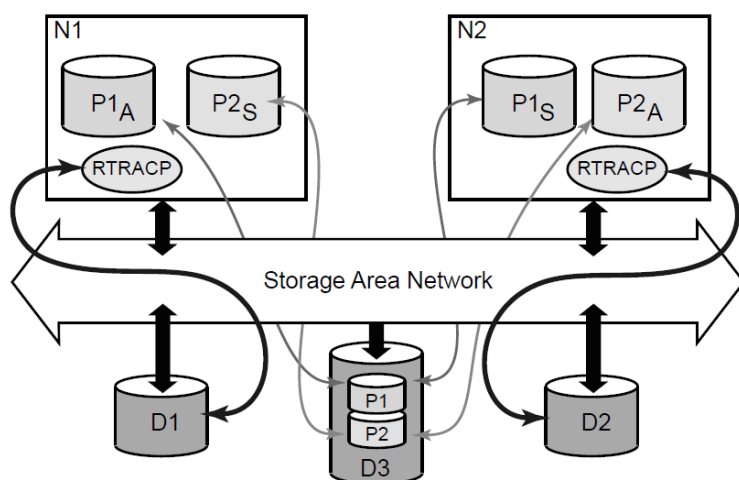
Figure 2.3. RTR Standby Servers
