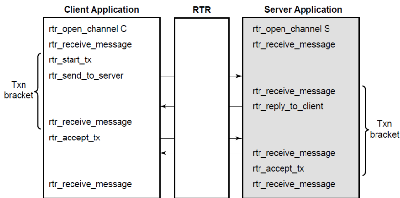
Figure 5.1. RTR C API Calls for Transactional Messaging
