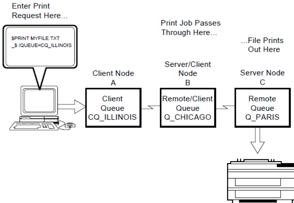
Figure 1.5. Daisy-Chained Queues
