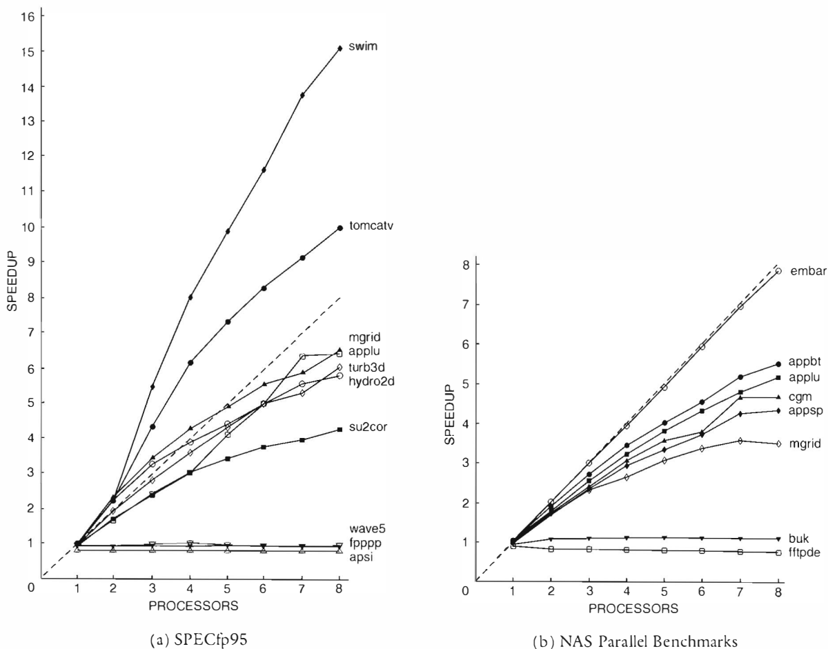
Figure 3 SUIF compiler speedups over the best sequential time achieved on the (a) SPECfp95 and (b) NAS parallel benchmarks.
