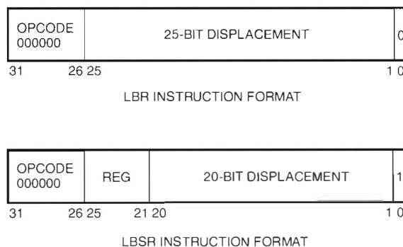
Figure 3 PALcode Long Branch Instruction Formats
