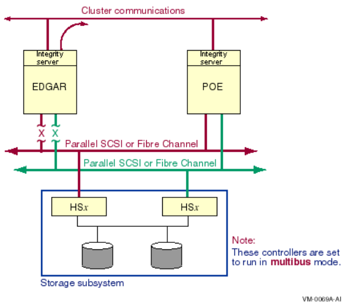
Figure 6.3. Direct SCSI to MSCP Served Configuration With Two Interconnects
