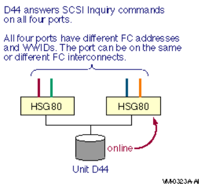
Figure 6.7. Port Addressing for Fibre Channel Controllers in Multibus Mode
