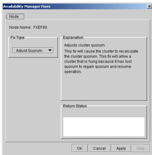
Figure 6.1. Adjust Quorum
