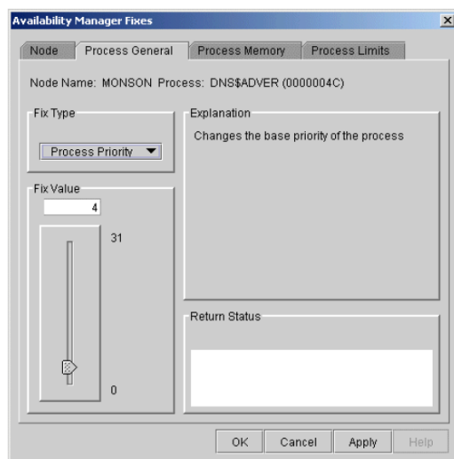
Figure 6.8. Process Priority
