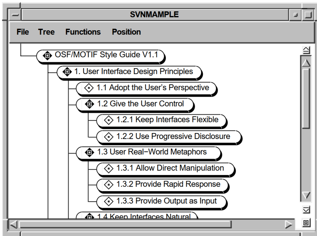
Figure 9.2. Tree Format
