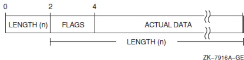
Figure 6.1. Segmented Records
