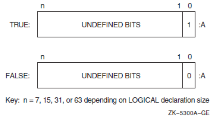
Figure 8.5. LOGICAL Representations
