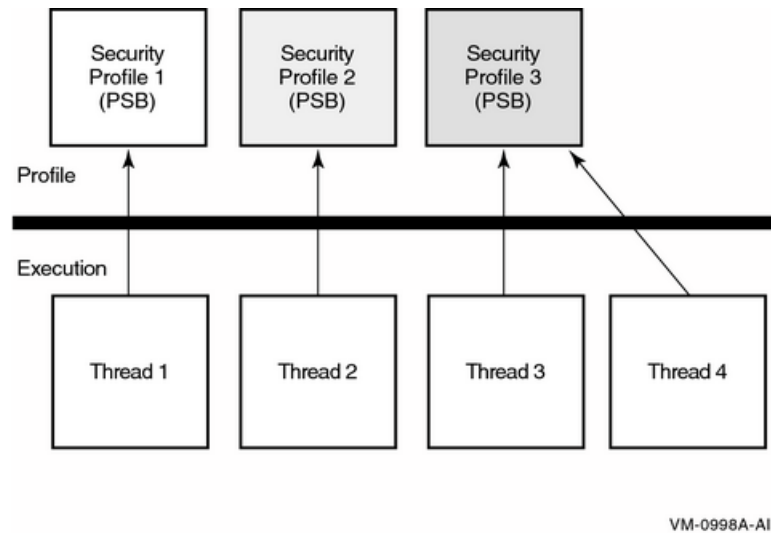
Figure 4.2. Per-Thread Security Profile Model
