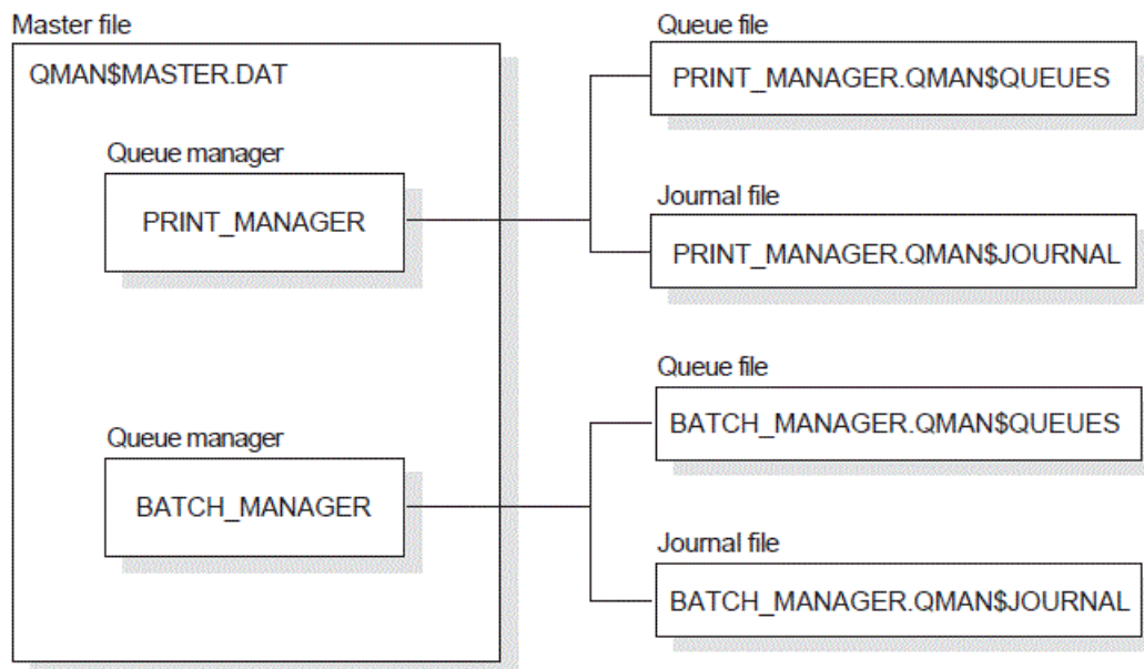
Figure 13.2. Queue Database
