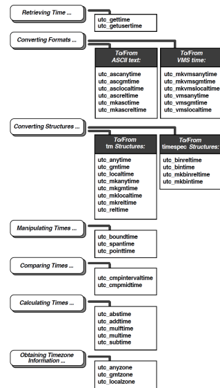
Figure 9.5. DTS Portable Interface Categories
