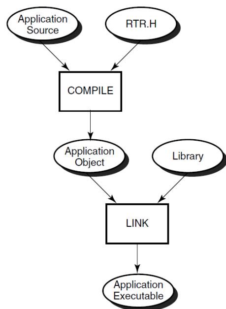
Figure 4.1. Compile Sequence
