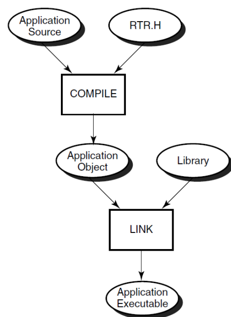
Figure 4.1. Compile Sequence
