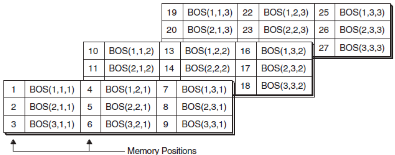
Three-Dimensional Array BOS (3,3,3)
