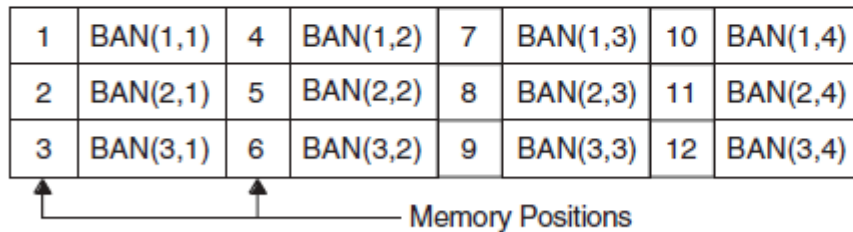
Two-Dimensional Array BAN (3,4)
