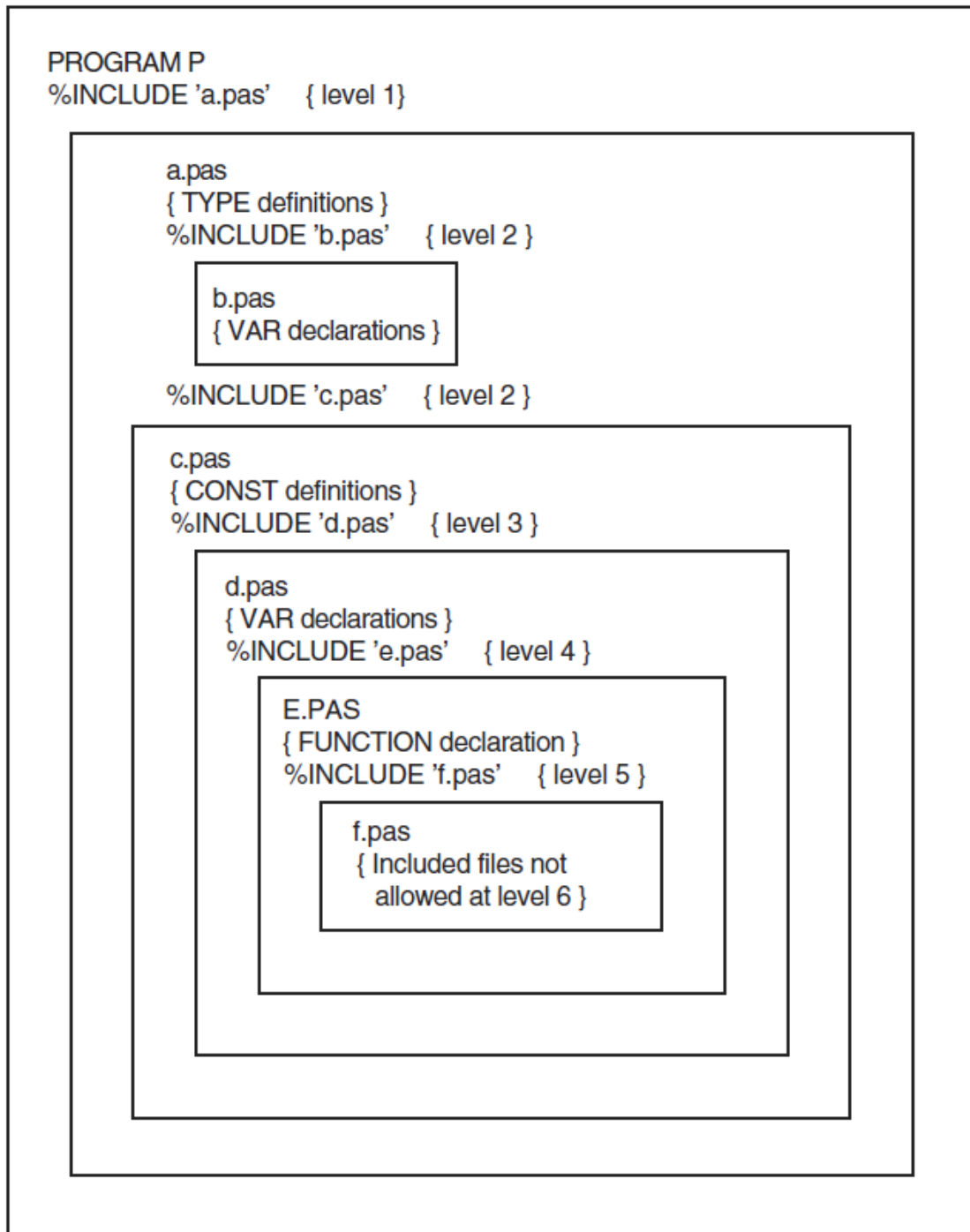
Figure 11.1. %INCLUDE File Levels
