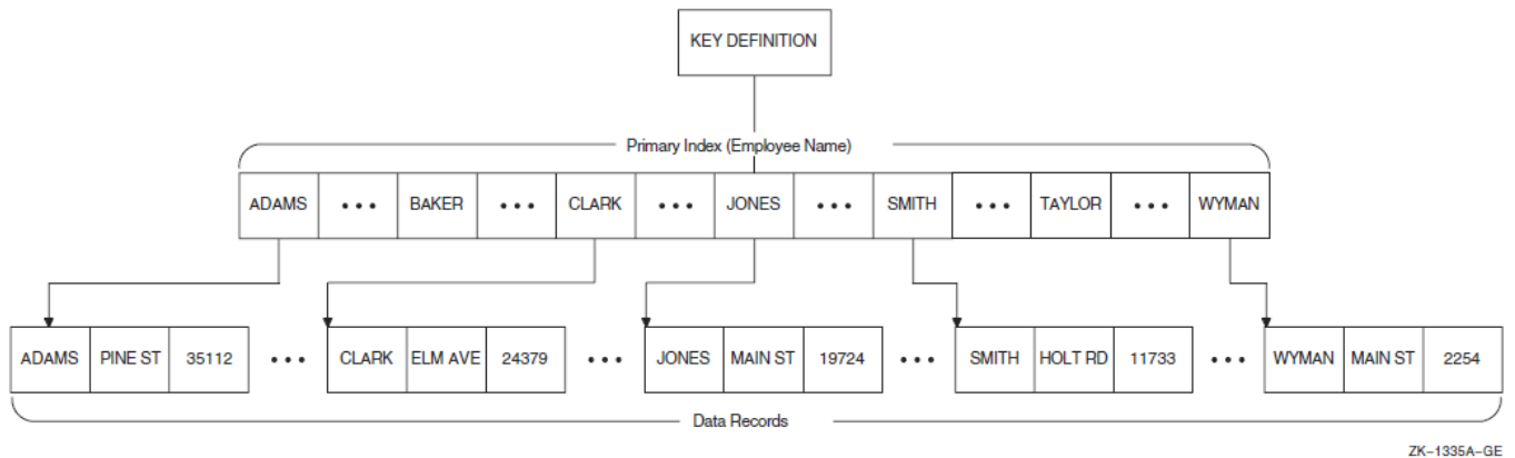
Figure 9.3. Indexed File Organization
