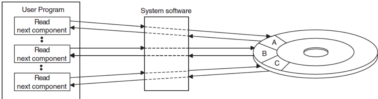
Figure 9.6. Sequential Access to a Sequential File
