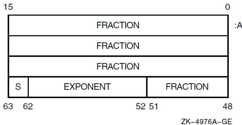
Figure A.6. T_floating-Point Data Representation
