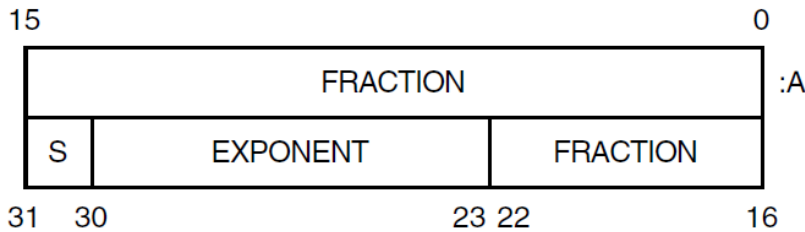
Figure A.3. S_floating-Point Data Representation
