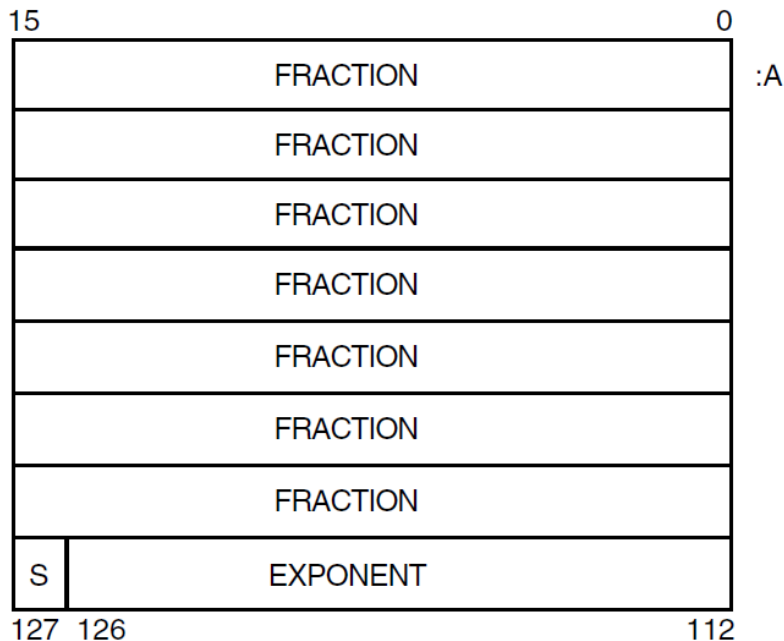
Figure A.8. X_floating-Point Data Representation
