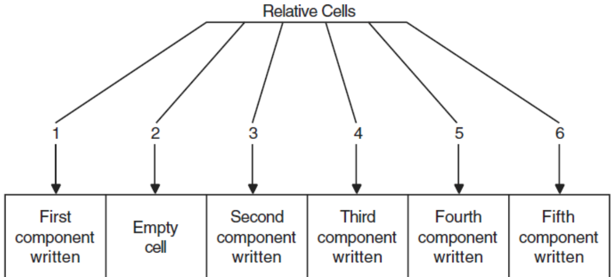
Figure 9.2. Relative File Organization
