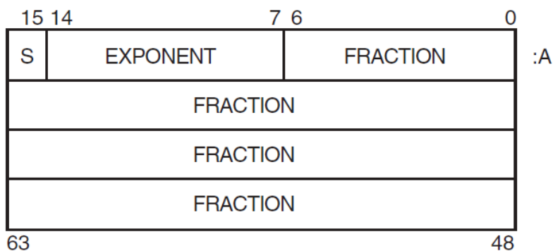
Figure A.4. D_floating-Point Data Representation
