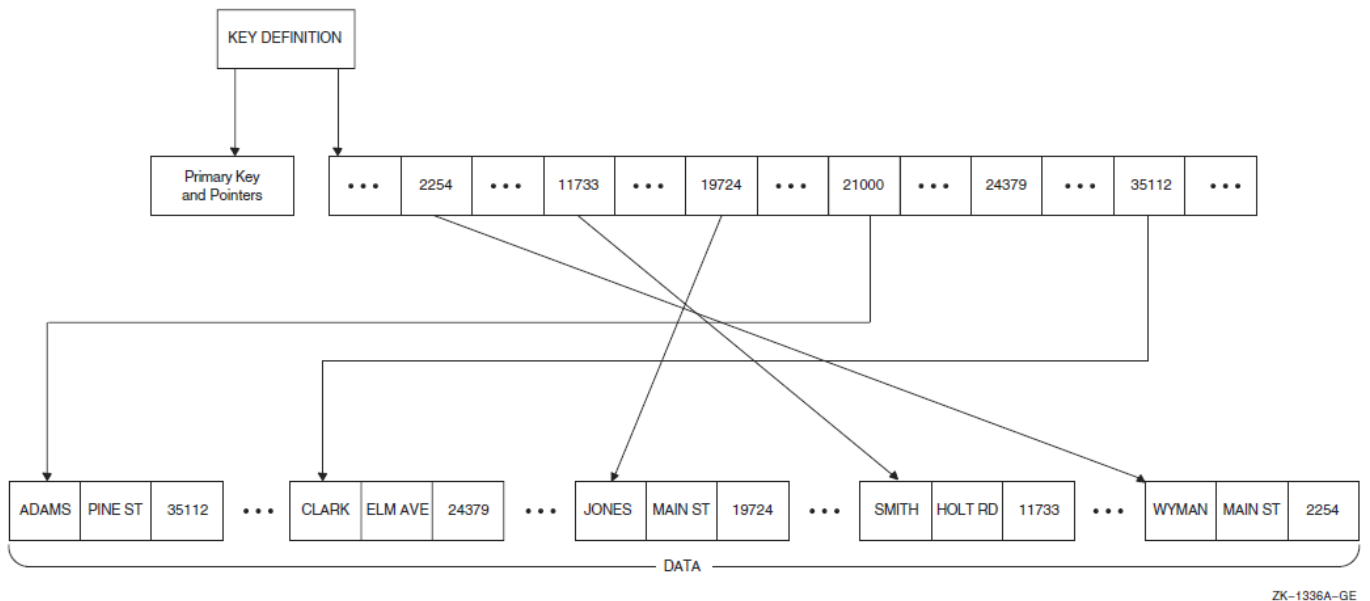
Figure 9.4. A First Alternate Key
