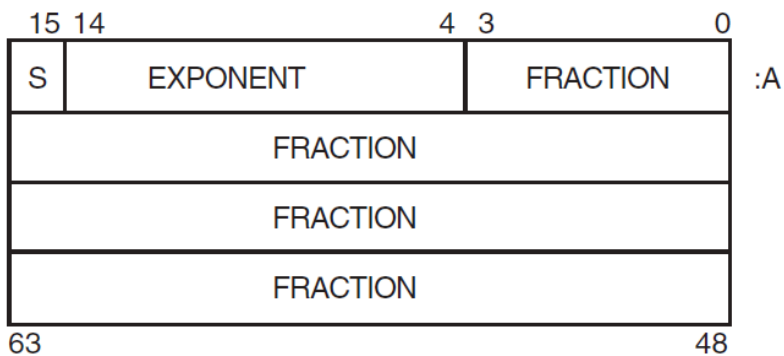
Figure A.5. G_floating-Point Data Representation
