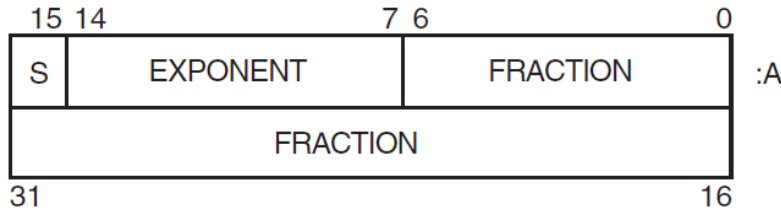
Figure A.2. F_floating-Point Data Representation
