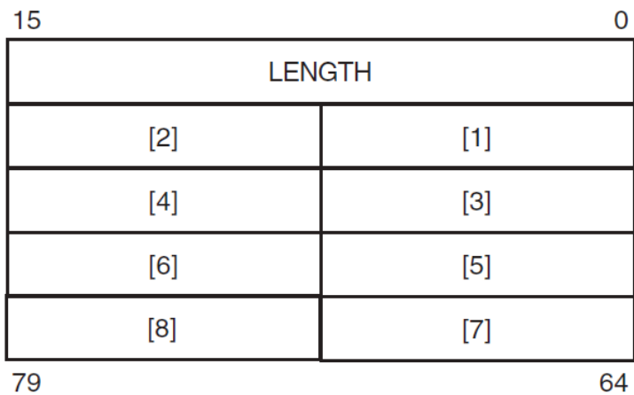
Figure A.1. Storage of Varying Data
