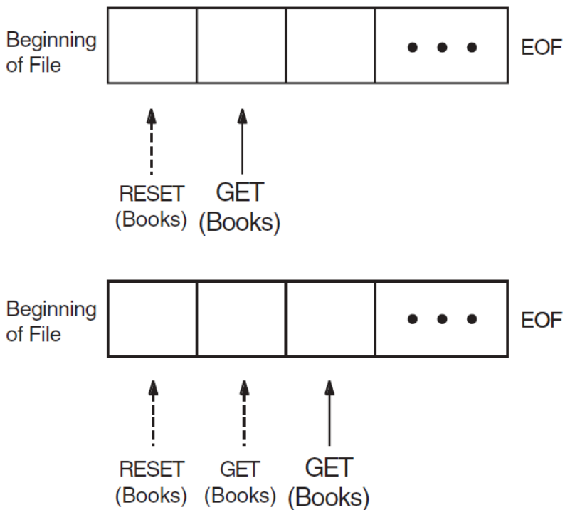
Figure 9.10. File Position After GET Procedure
