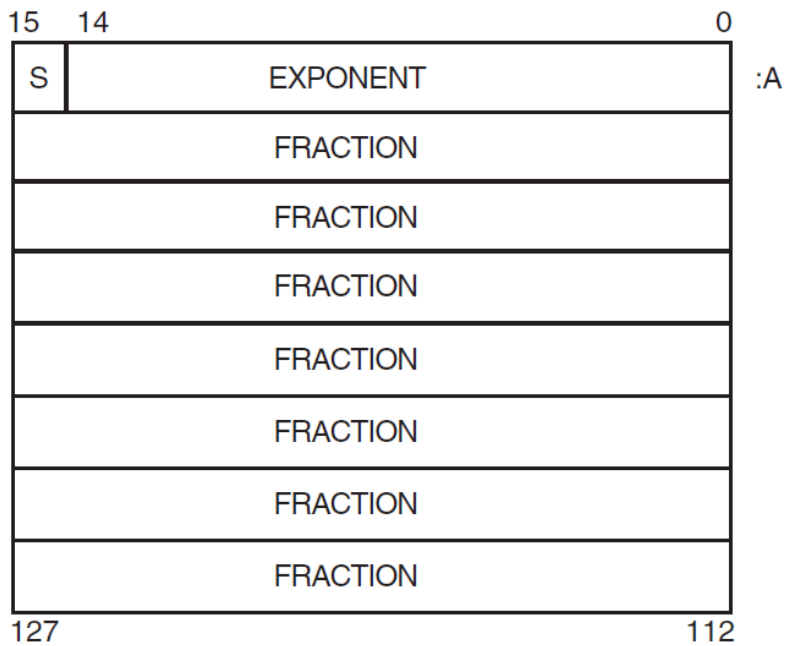
Figure A.7. H_floating-Point Data Representation
