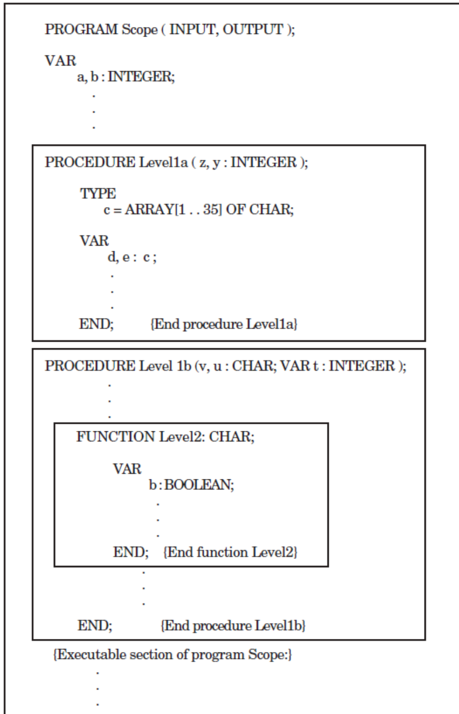
Figure 7.1. Scope of Identifiers
