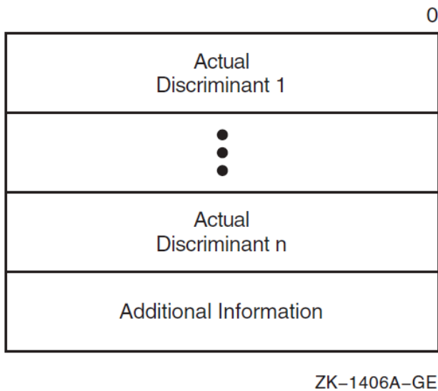
Figure A.9. Storage of Nonstatic Data Types
